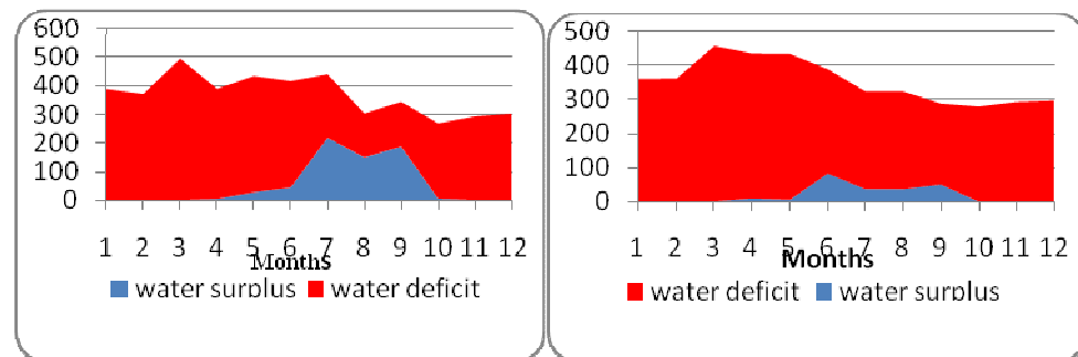
Figure.5.3. Niamey Water Balance in 1999 Figure.5.4. Niamey Water Balance in 2000
