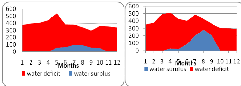
Figure. 5.1, Niamey Water balance in 1997 Figure.5.2, Niamey Water Balance in 1998
