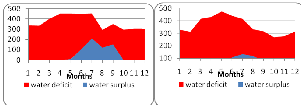
Figure. 5.5 Niamey Water Balance in 2001 Figure 5.6 Niamey Water Balance in 2002
