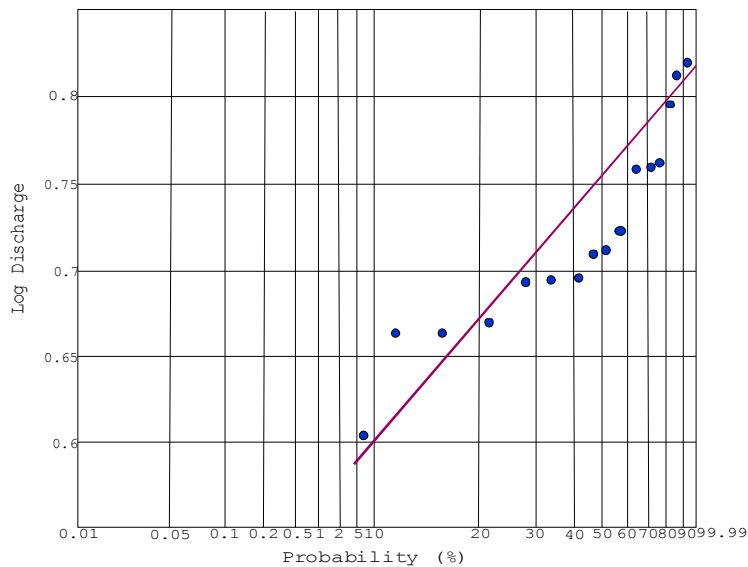
Figure 6: 7-Day Low Flow Frequency Curve
